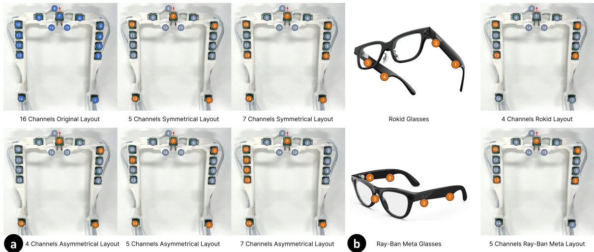
Fig. 18. Liveness detection and authentication accuracy were evaluated under limited input-channel settings. (a) Top row shows the original microphone layout of the prototype and the selected microphones for the 5- and 7-channel symmetric configurations. Bottom row shows the selected microphones for the 4-, 5-, and 7-channel asymmetric configurations. Selected microphones are highlighted in orange. (b) demonstrates the microphone layouts of Rokid Glasses and Ray-Ban Meta Glasses on the left, and the microphones used in our experiments to simulate their recording characteristics on the right, with selected microphones highlighted in orange.
