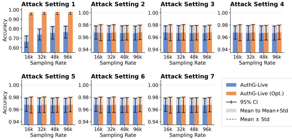
Fig. 14. Liveness detection accuracy under different sampling rates. Note: Optimization is described in Section 5.3.
