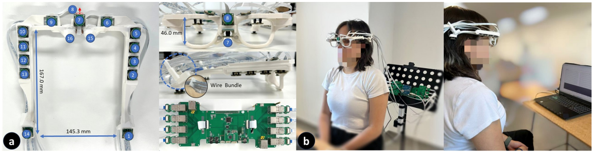
Fig. 7. (a) Structural and hardware overview of the prototype. The system comprises 14 air-conduction microphones and 2 bone-conduction microphones. Each microphone is connected to the data collection board via flexible flat cables, and the temple is designed with a wire bundle, which can reduce crosstalk between channels. (b) Illustration of a user wearing the smart glasses prototype.
