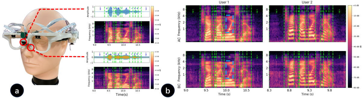
Fig. 4. This figure illustrates the air-conductive (AC) and bone-conductive (BC) microphones used for feature selection. (a) The raw audio signals and corresponding Mel-spectrograms captured by AC and BC microphones when a user speaks the phrase “check my voicemail.” The utterance is segmented into phonemes. The results show that both AC and BC microphones capture rich time–frequency characteristics. (b) Comparison of air-conducted (AC) and bone-conducted (BC) signals from different users uttering “check my voicemail,” visualized using a consistent color scheme. As highlighted by the blue boxes, AC and BC signals from the same user exhibit subtle frequency-related differences, whereas signals captured by either AC or BC microphones show pronounced inter-user variability.
