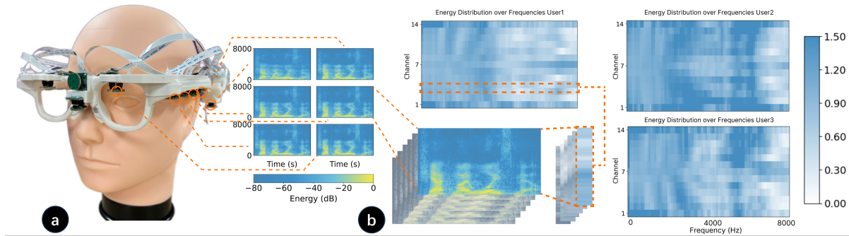
Fig. 6. This figure illustrates the computation of Energy Distribution over Frequencies (EDF) and the spatial acoustic information it captures. (a) STFT of signals recorded by microphones at different positions on the glasses. (b) For each microphone, the STFT is averaged along the time axis to obtain the energy–frequency representation. On the right, EDFs for different users uttering the phrase “check my voicemail” are shown, highlighting inter-user variations.
