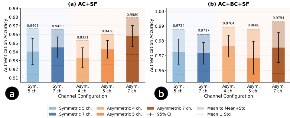
Fig. 17. Authentication accuracy under different channel inputs (1) without and (2) with BC modality.
