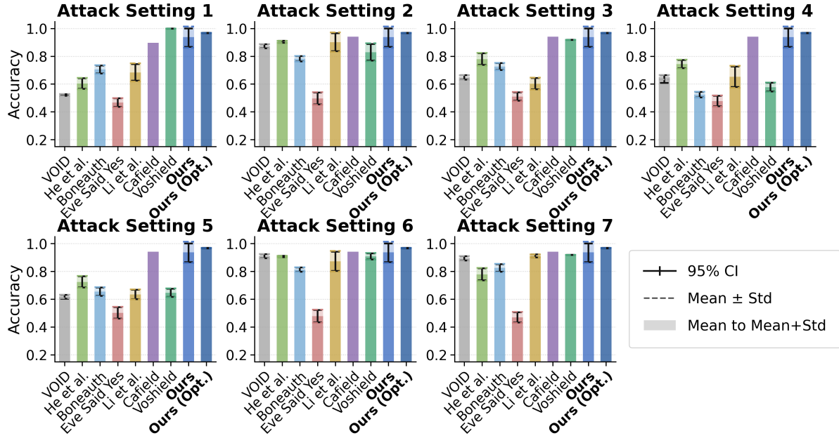
Fig. 12. Result for benchmark task 2. Note: (1) optimization for our method is described in section 5.3; (2) As our method do not require attack samples for training, we average the liveness detection accuracy on all attacks.
