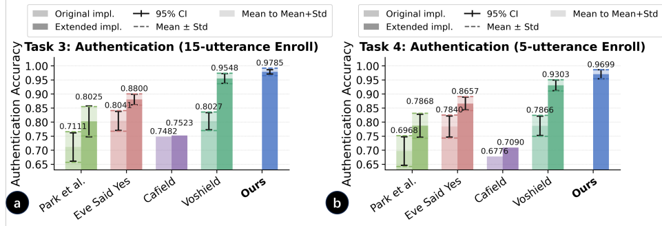
Fig. 13. (a) Result for benchmark task 3. (b) Result for benchmark task 4.
