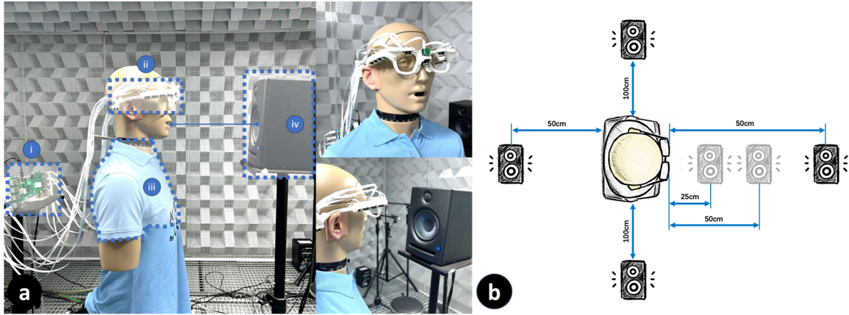
Fig. 8. (a) The environment setting of the voice attack. i is the data collection board and ii is the smart glasses frame. All microphones are connected via bundled flexible flat cables to a data collection board. iii is the torso-mouth simulator and iv is the loudspeaker. In the experiment, two types of replay sample were applied: loudspeaker replay and a torso-mouth simulator replay which replicates the exhalation process and torso vibrations during speaking. (b) In the replay attack, the loudspeaker was placed at different positions and distances from the smart glasses to simulate various attack situations.
