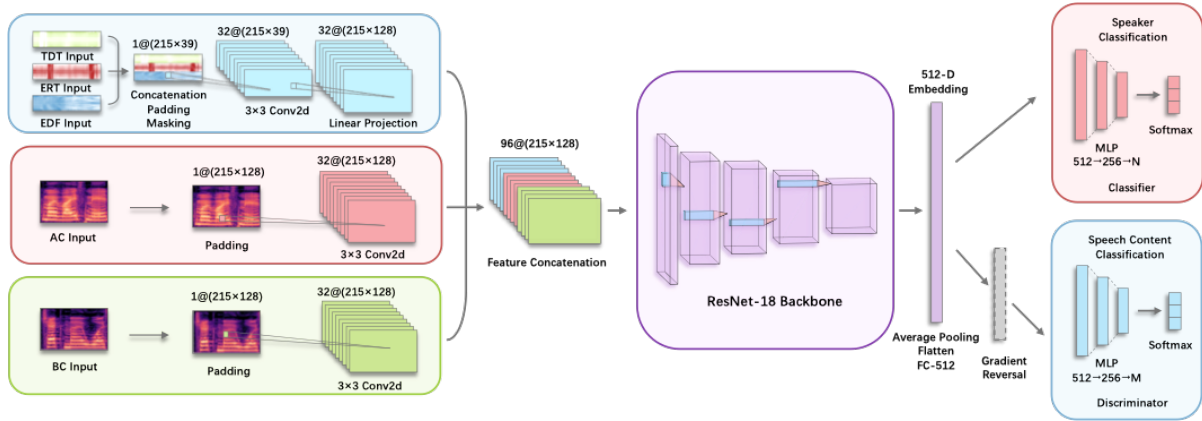
Fig. 10. The figure demonstrate the architecture of AuthG-Net. The blue/red/green blocks on the left denote the SF/AC/BC inputs, which are encoded by lightweight CNN heads and then stacked and fed into a ResNet-18 backbone (purple block) to produce a 512-D embedding. In the domain-adversarial learning (DAL) branch, the model is optimized with two objectives: speaker classification (red) and speech-content classification (blue). The speaker classifier is trained directly on the embedding, whereas the passphrase classifier is connected via a Gradient Reversal Layer (GRL), which reverses gradients during backpropagation to encourage content-invariant embeddings.
