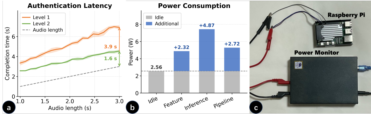
Fig. 21. Live system overhead. (a) Authentication latency vs. audio length for the two simplification levels (shaded: \pm 1 std over 5 repeats); the gap to the dashed audio length line is the processing latency (3.9 s for Level 1 and 1.6 s for Level 2 at 3 s input). (b) Power on the Raspberry Pi: idle baseline (2.56 W, dashed) plus the additional power per 3-second segment; the memory footprint stays below 267 MB. (c) The power-measurement setup.
