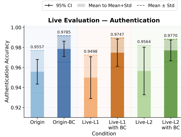
Fig. 23. Authentication accuracy under two levels of simplification.
