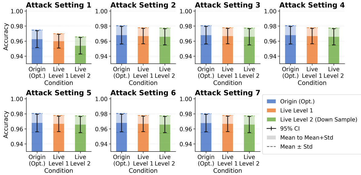
Fig. 22. Liveness detection accuracy under two levels of simplification.
