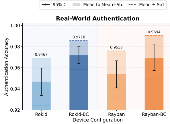
Fig. 20. Authentication accuracy for Rokid and Ray-ban Meta configurations.
