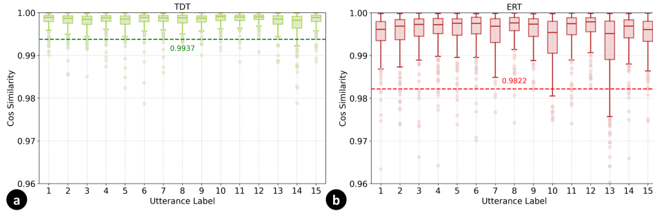
Fig. 9. This figure shows the distribution of cosine similarities between the unified patterns and the corresponding aTDT and aERT across all genuine samples for the 15 utterances. Each box in the boxplot represents the interquartile range (25th to 75th percentile), with the line inside indicating the median. Scattered points denote outliers, and the dashed line marks the 3rd percentile of the genuine similarity distributions. In (a), the TDT cosine similarity between aTDT and the unified patterns defines a threshold of 0.9937, whereas in (b), the ERT yields a threshold of 0.9822.
