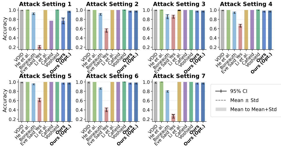
Fig. 11. Result for benchmark task 1. Note: (1) optimization (Opt.) for our method is described in section 5.3; (2) Since the other methods are trained and evaluated using known attack types, they may be prone to overfitting to specific attacks. In contrast, our method determines the decision threshold using only genuine samples and demonstrates superior performance under unseen attack scenarios, as discussed in Section 4.4.2.
