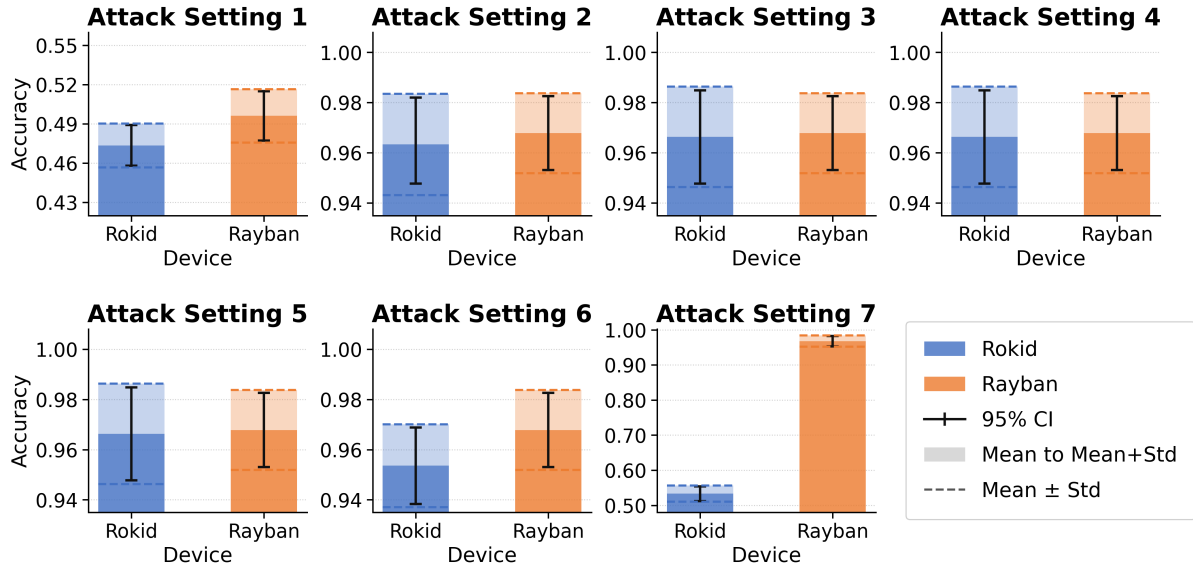
Fig. 19. Liveness detection accuracy for Rokid and Ray-ban Meta configurations.
