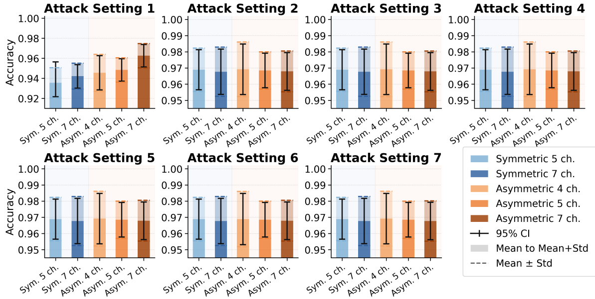
Fig. 16. Liveness detection accuracy under different channel inputs.
