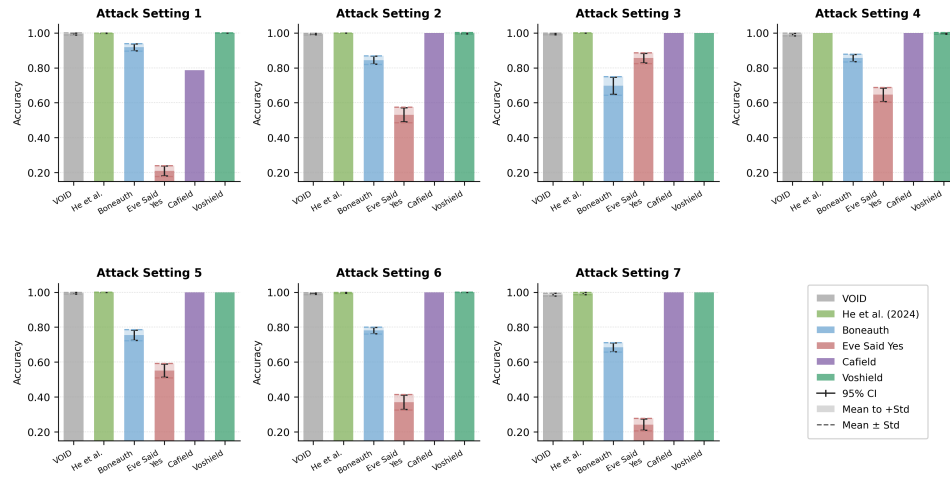
Fig. 25. Liveness detection accuracy for original baseline implementation.
