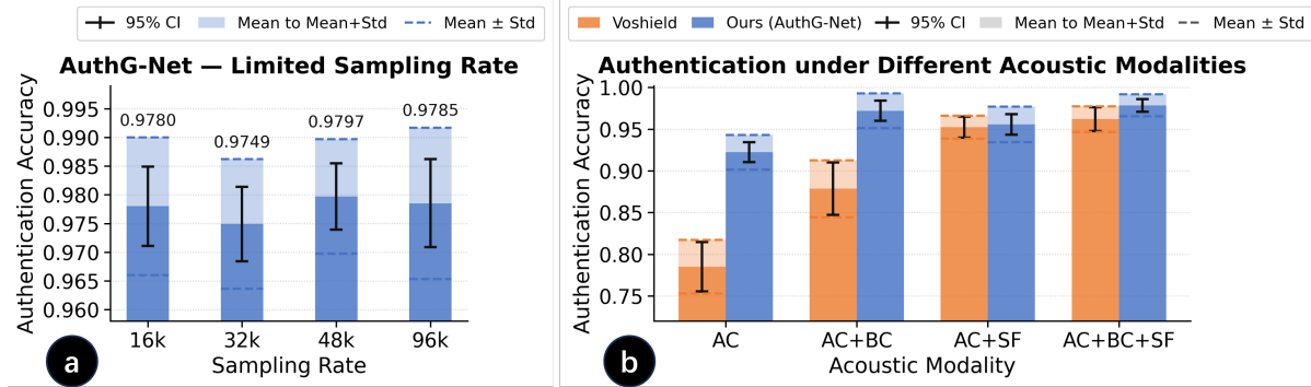
Fig. 15. (a) Authentication accuracy under different sampling rates. (b) Authentication accuracy under different input modalities.
